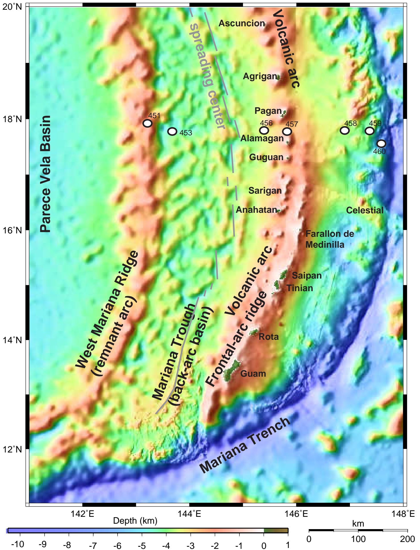
Figure 4. Bathymetry and geologic elements of Mariana arc system. After Taylor (UofH)/Klemperer (Stanford)/Wiens (WUSTL)/Hildebrand (SIO) proposal to NSF-MARGINS, January 2000.
